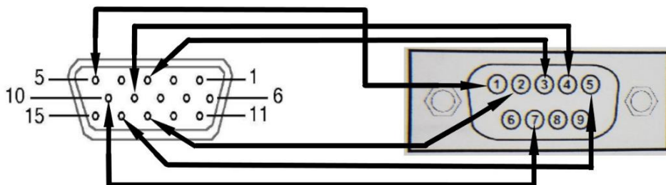
Figure 8 - Elecraft K3 Accessory Jack Interface - as viewed from the rear panel
